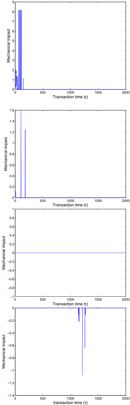
FIG. 2: Examples of mechanical price impact (in pence) in transaction time. The top two plots correspond to buy orders and the bottom two to sell orders.
