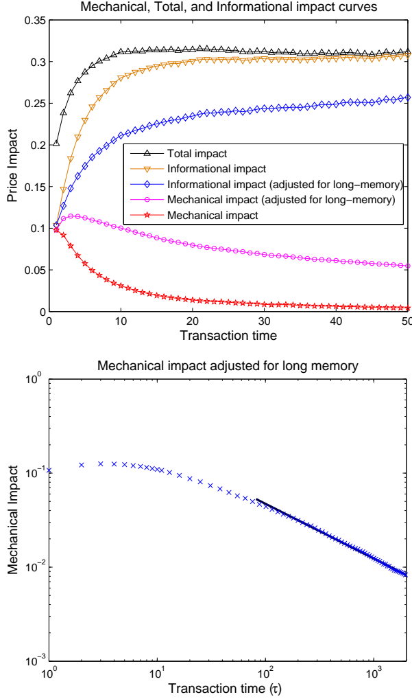
FIG. 8: (a) A comparison of the average mechanical, informational, and total impacts with and without adjustments for long-memory. In ascending order we show the average mechanical impact R^M(\tau) , the mechanical impact C(\tau) adjusted for long-memory, the informational impact adjusted for long-memory R^T(\tau) - C(\tau) , the informational impact R^T(\tau) - R^M(\tau) , and the total impact R^T(\tau) , all as a function of time. In (b) we show C(\tau) over a longer time period in double logarithmic scale.
