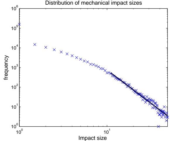
FIG. 6: The distribution of integrated mechanical impact sizes S_{\tau}^M(t) , with \tau = 2000 . The x's are the real data and the solid line is a fit to a power law. The units of the x axis are price \times time, where price differences are measured in units of average spread and time is measured in transactions.
