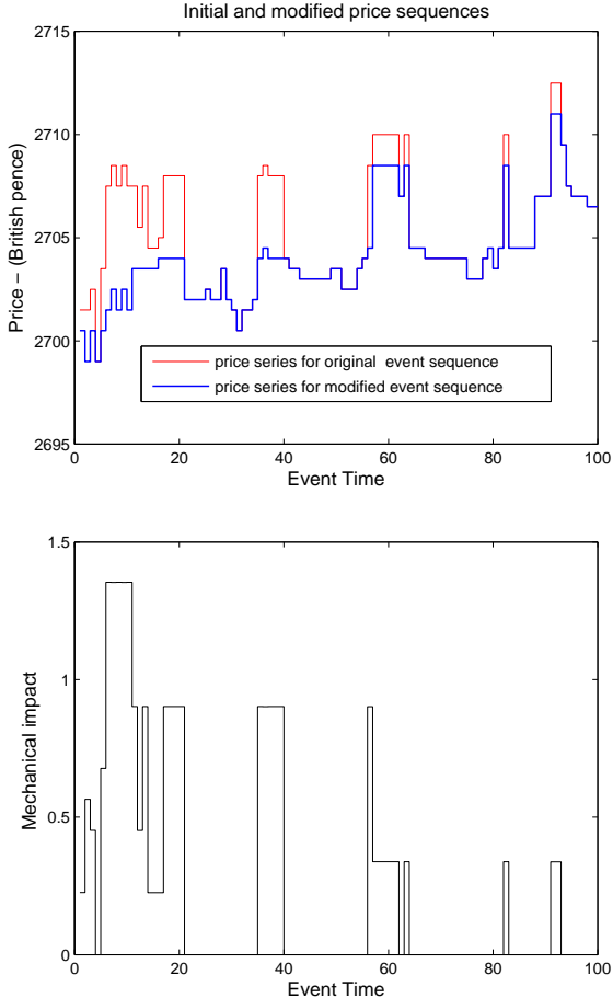
FIG. 1: (a) Initial and modified price sequences for the removal of a buy market order and (b) the resulting mechanical impact (which is just the difference between the two price series in (a)). Note that this figure and all other figures in this paper are based on the stock AZN. Prices are in pence.
