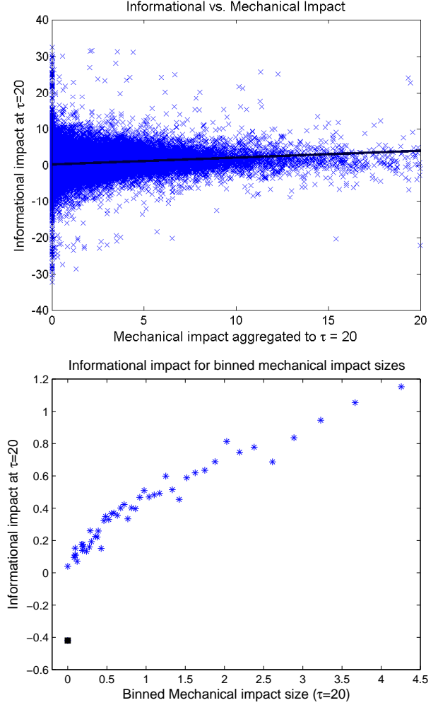
FIG. 9: The informational impact at \tau = 20 vs. mechanical impact integrated up to \tau = 20 , S_{20}^M(t) . In (a) the dots correspond to individual transactions, and the line is a regression using ordinary least squares. In (b) the data is binned based on the integrated mechanical impacts, illustrating that even though the relationship is noisy, the correlation increases consistently with increasing size. Note that the black square corresponds to the case where the mechanical impact is strictly zero.
