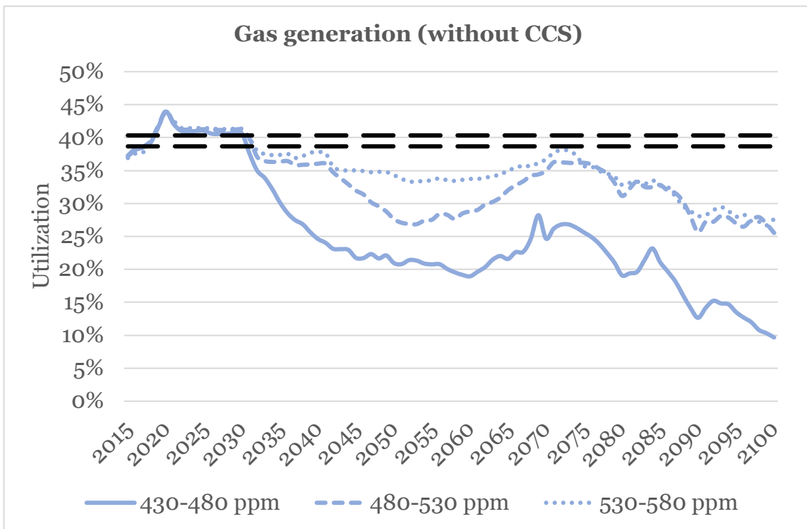
Figure 1: Simulation results for coal- and gas-fired capacity utilization. (a) coal
