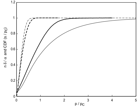
FIG. 19: Fit of the self-consistent solution with diffusivity term to simulation results for the midpoint-centered frame. Thin solid line is the analytic solution for the mean number density, and thick solid line is simulation result, at \epsilon = 0.02 . Thin dashed line is the analytic prediction for the cumulative distribution function \Pr(\hat{s}/2 \leq \hat{p}) , and thick dashed line is simulation result.
