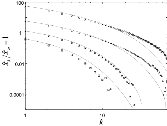
FIG. 25: Four pairs of curves for the quantity \hat{x}_k/\hat{x}_\infty - 1 vs. k . The value of \epsilon increases from top to bottom ( \epsilon = 0.02, 0.04, 0.2, 0.66 ). In each pair of curves, the markers are obtained from simulations while the solid curve is the prediction of Eq. 53 evaluated numerically. The difference between numerics and mean-field increases as \epsilon decreases, especially for large k .
