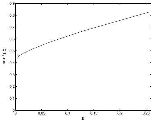
FIG. 10: The mean value of the spread in nondimensional units \hat{s} = s/p_c as a function of \epsilon . This demonstrates that the spread only depends weakly on \epsilon , indicating that the prediction from dimensional analysis given in table (III) is a reasonable approximation.
