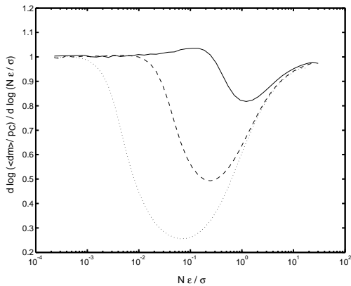
FIG. 8: Derivative of the nondimensional mean mid-price movement, with respect to logarithm of the nondimensional order size N/N_c = N\epsilon/\sigma , obtained from the price impact curves in Fig. 6.
