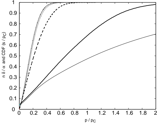
FIG. 21: Reconstruction with correlated source terms for \epsilon = 0.02 . Line style and thickness are the same as in Fig. 20.
