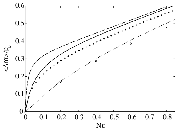
FIG. 27: Three pairs of curves for the quantity \langle \Delta m \rangle / p_c vs. N\epsilon where \langle \Delta m \rangle = 1/2 \sum_{k=1}^N x_k . The value of \epsilon increases from top to bottom ( \epsilon = 0.002, 0.02, 0.2 ). In each pair of curves, the markers are obtained from simulations while the solid line is the prediction of the IIA. For \epsilon = 0.002 , we show only the theoretical prediction. The theory captures the functional form of the price impact curves for different \epsilon . Quantitatively, it's better for larger epsilon, as remarked earlier.
