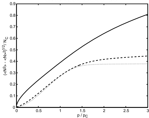
FIG. 4: Standard deviation of the nondimensionalized cumulative depth versus nondimensional price, corresponding to Fig. (3).
