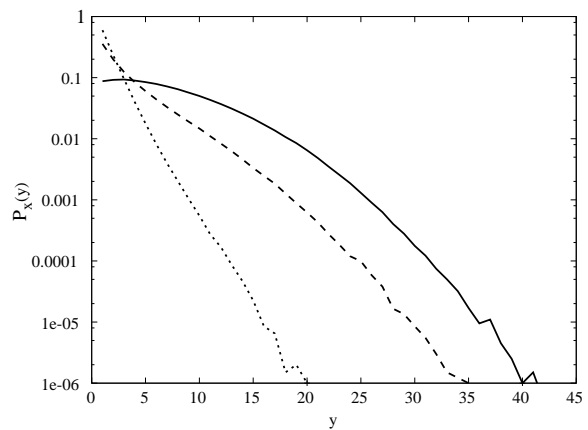
FIG. 23: The probability distribution functions P_x(y) vs. y for the intervals x = x_0, x_1 and x_5 at \epsilon = 0.1 , on a semi-log scale. Solid curve is for x_0 , dashed for x_1 , and dot for x_5 . The functional form of the distribution changes from a Gaussian to an exponential.
