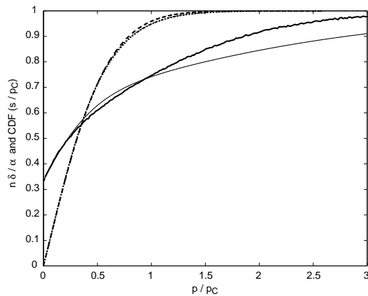
FIG. 20: Reconstruction with source terms \mathcal{S} that approximately account for correlated fluctuations near the midpoint. \epsilon = 0.2 . Thick solid line is averaged order book depth from simulations, and thin solid is the mean field result. Thin dotted line is the simulated CDF for \hat{s}/2 , and thick dotted line is the mean field result. Thick dashed line is the CDF that would be produced from the simulated depth, if the mean-field approximation were exact.
