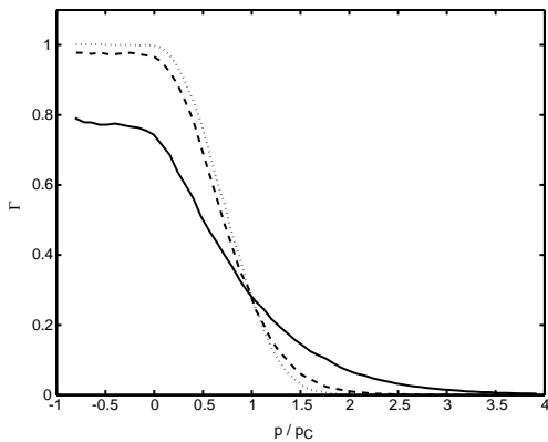
FIG. 12: The probability \Gamma for filling a limit order placed at a price p/p_c where p is calculated from the instantaneous mid-price at the time of placement. The three cases correspond to Fig. 3: \epsilon = 0.2 (solid), \epsilon = 0.02 (dash), \epsilon = 0.002 (dot).
