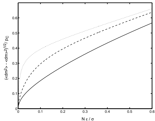
FIG. 7: The standard deviation of the instantaneous price impact dm/p_c corresponding to the means in Fig. 6, as a function of normalized order size \epsilon N/\sigma . \epsilon = 0.2 (solid), \epsilon = 0.02 (dash), \epsilon = 0.002 (dot).
