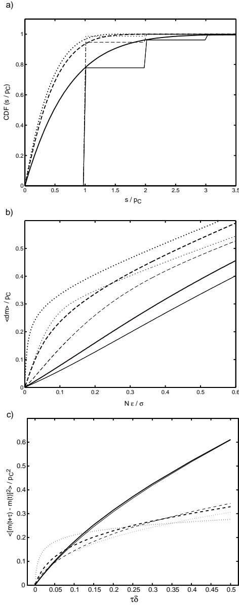
FIG. 14: Dependence of market properties on tick size. Heavy lines are dp/p_c \rightarrow 0 ; light lines are dp/p_c = 1 . Cases correspond to Fig. 3, with \epsilon = 0.2 (solid), \epsilon = 0.02 (dash), \epsilon = 0.002 (dot). (a) is the cumulative distribution function for the nondimensionalized spread. (b) is instantaneous nondimensionalized price impact, (c) is diffusion of the nondimensionalized midpoint shift, corresponding to Fig. 11.
