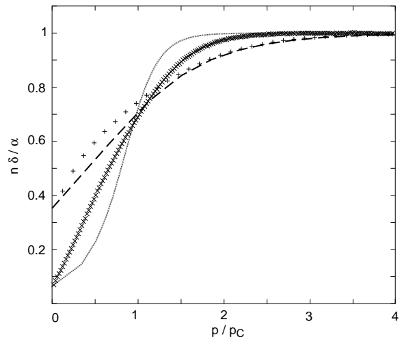
FIG. 29: Density profiles from Monte Carlo simulation (markers) and the Independent Interval Approximation (lines). Pluses and dash line are for \epsilon = 0.2 , while crosses and dotted line are for \epsilon = 0.02 .
