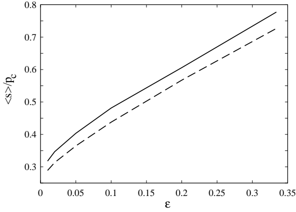
FIG. 24: The mean value of the spread in nondimensional units \hat{s} = s/p_c as a function of \epsilon . The numerical value above (solid) is compared with the theoretical estimate below (dash).
