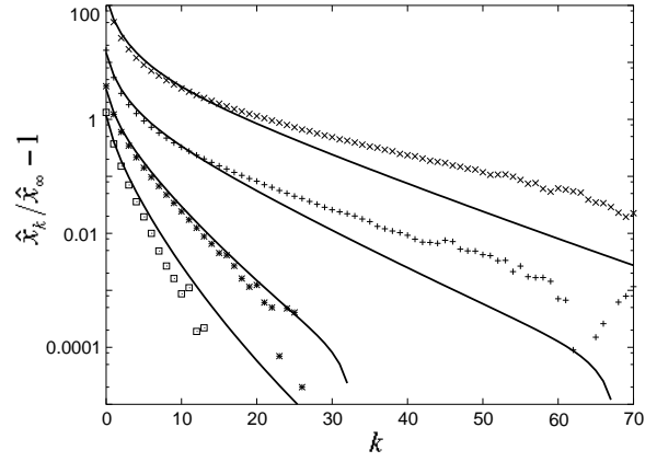
FIG. 26: Same plot as Fig. 25 but on a semi-log scale to show exponential decay at large k .
