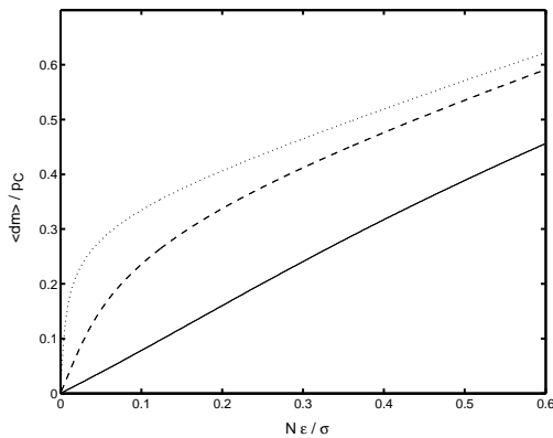
FIG. 6: The average price impact corresponding to the results in Fig. (3). The average instantaneous movement of the nondimensional mid-price, \langle dm \rangle / p_c caused by an order of size N/N_c = N\epsilon/\sigma . \epsilon = 0.2 (solid), \epsilon = 0.02 (dash), \epsilon = 0.002 (dot).
