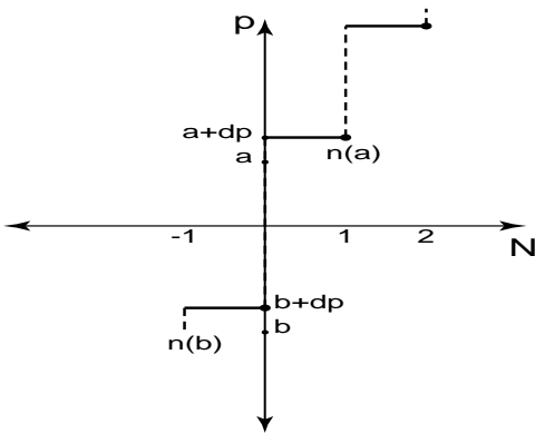
FIG. 17: The inverse function p(N, t) . The function is in general defined only on discrete values of N , so this domain is only invariant when order size is fixed, a convenience that will be assumed below. Between the discrete domain, and the definition of p as a maximum, the inverse function effectively interpolates between vertices of the reflected image of N(p, t) , as shown by the dotted line.
