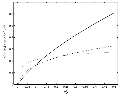
FIG. 11: The variance of the change in the nondimensionalized midpoint price versus the nondimensional time delay interval \tau\delta . For a pure random walk this would be a straight line whose slope is the diffusion rate, which is proportional to the square of the volatility. The fact that the slope is steeper for short times comes from the nontrivial temporal persistence of the order book. The three cases correspond to Fig. 3: \epsilon = 0.2 (solid), \epsilon = 0.02 (dash), \epsilon = 0.002 (dot).
