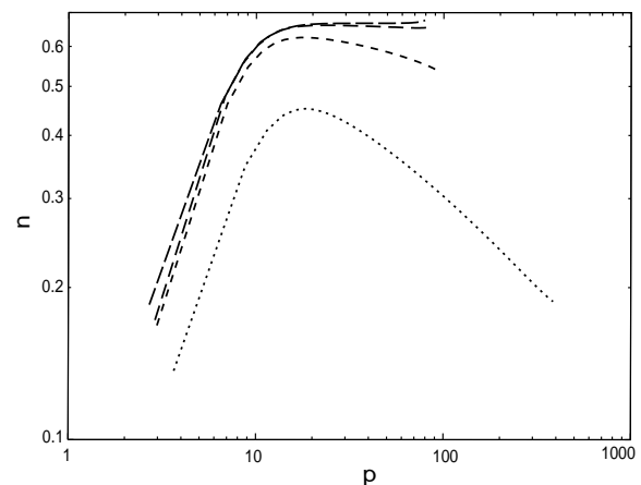
FIG. 30: Density profiles for a power-law order placement process for different values of \Delta_0 .
