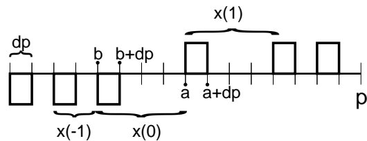
FIG. 15: The price space and order profile. n(p, t) has been chosen to be 0 or \pm 1 , a restriction that will be convenient later. Price bins are labeled by their lower boundary price, and intervals x(N) will be defined below.
