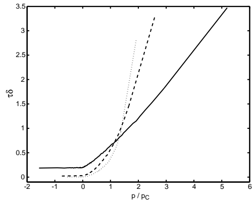
FIG. 13: The average time \tau nondimensionalized by the rate \delta , to fill a limit order placed at a distance p/p_c from the instantaneous mid-price.
